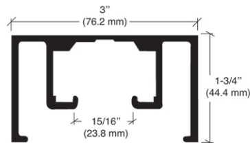
D1670 OVERHEAD TRACK When Matching a Store Front Extrusion, D1670 Upper Track may be used. Specify D1028 Assembly
