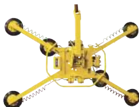
CAT. NO. MRTA611LDC Lifting Capacity: 1,100 lbs. (500 kg)
