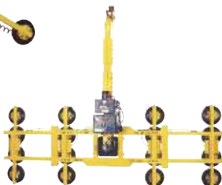
CAT. NO. MR1611LDC Lifting Capacity: 2,800 lbs. (1270 kg)
