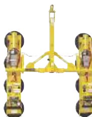
CAT. NO. P2110445DC Lifting Capacity: 1,400 lbs. (635 kg)
